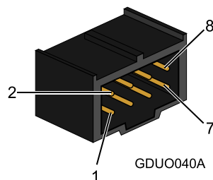
8-Pin 2.54 mm Pitch Molex
