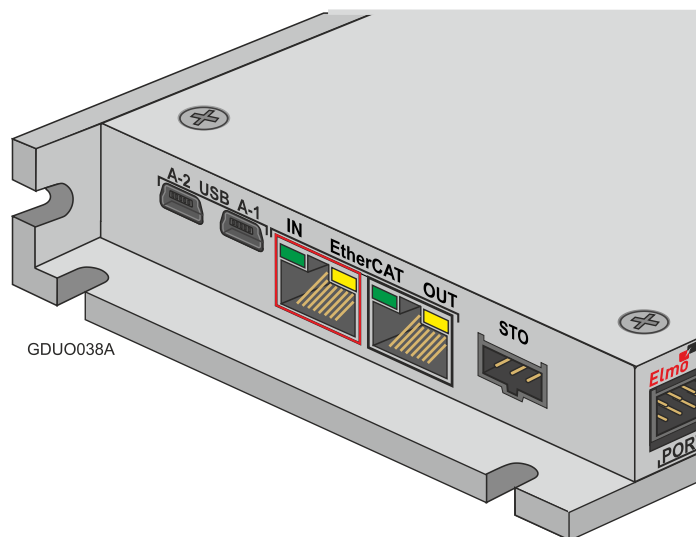
8-Pin RJ-45
