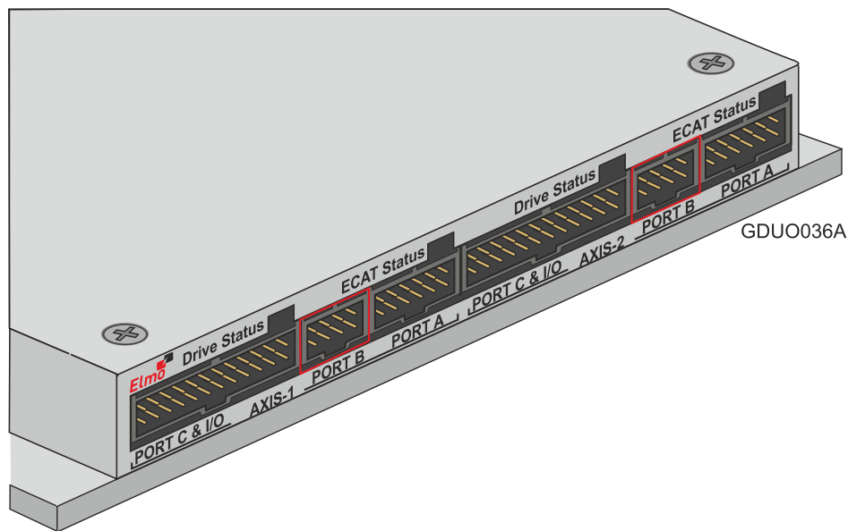
8-Pin Molex Plug
